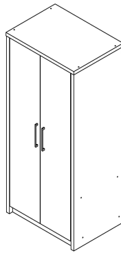
Wardrobe W800 x D580 x H1830mm
