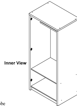
Wardrobe W800 x D580 x H1830mm
