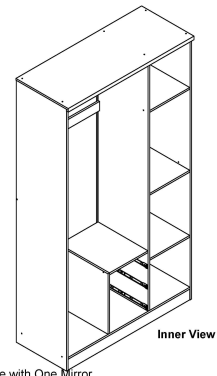
3 Door / 3 Drawer Wardrobe with One Mirror W1200 x D500 x H1820mm
